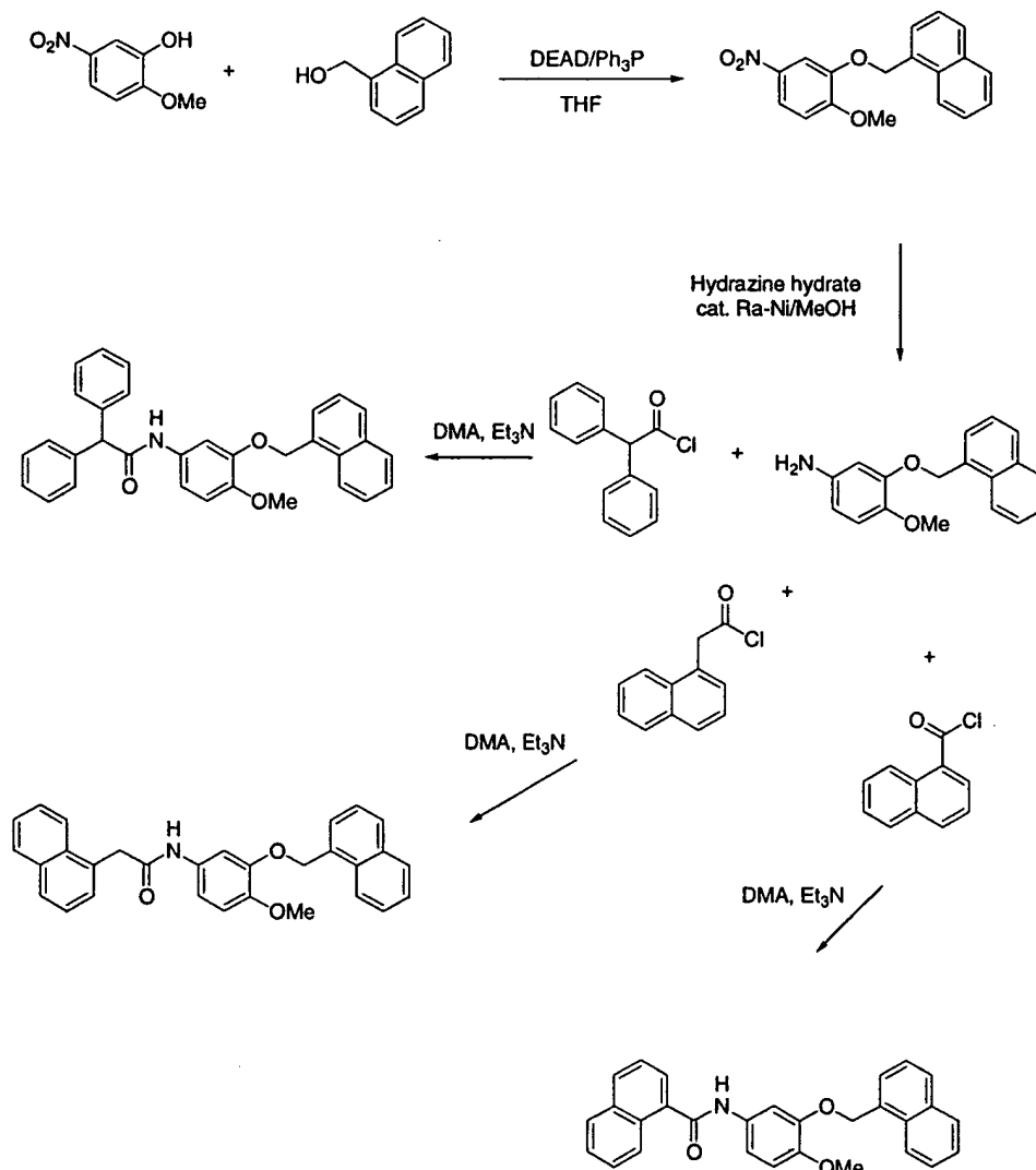
Scheme XIII
